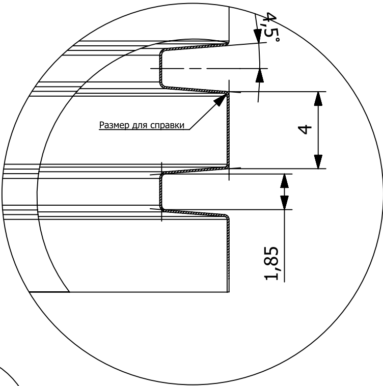
DETAIL A SCALE 5:1
