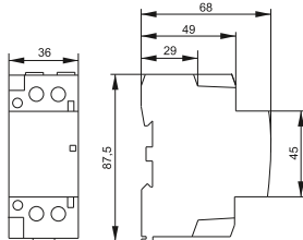
Контакторы KM63-20M AC, KM63-11M AC, KM40-20M AC и KM40-11M AC
