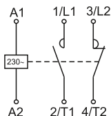
KM20-11M AC, KM40-11M AC, KM63-11M AC
