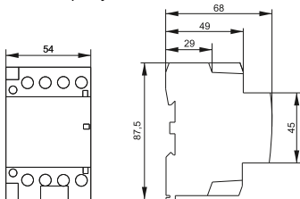
Контакторы KM25-40M AC/DC, KM40-40M AC/DC и KM63-40M AC/DC
