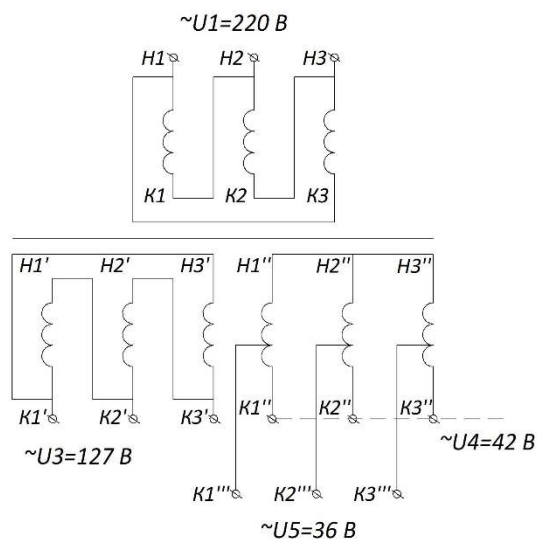
ТС3И-(1,6-2,5-4,0)-220/127;42;36
