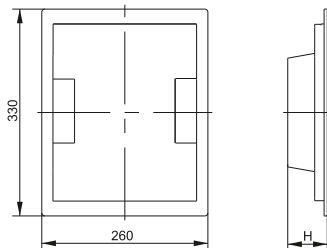
Рисунок 1 – Лючок ONFLOOR / Figure 1 – Hatch ONFLOOR / 1-suret – ONFLOOR lügy
