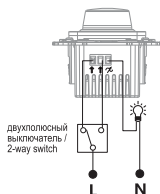
b) FI-D23-0550-P-X*; FI-D22-0250-P-X* (проходной / pass-through / өтпелі)
