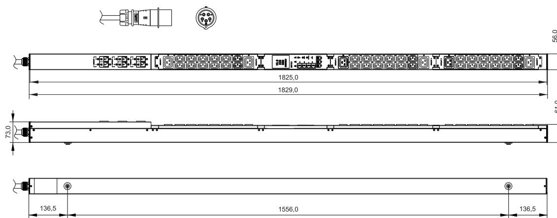
Рисунок 6 – AN-PM13-42-36C13-06C19-43, CN-PM23-42-36C13-06C19-43, AN-PM33-42-36C13-06C19-43, CN-PM43-42-36C13-06C19-43
