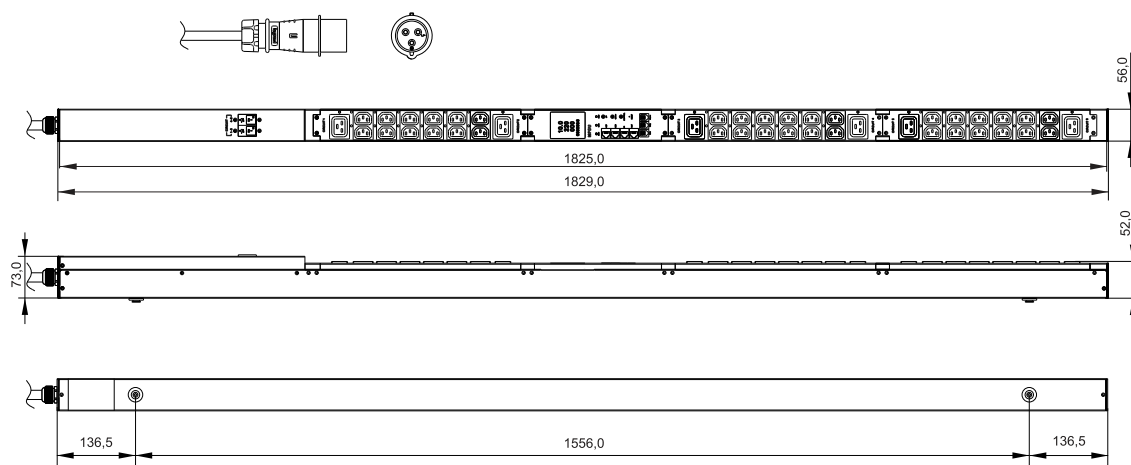
Рисунок 4 – AN-PM13-42-36C13-06C19-41, CN-PM23-42-36C13-06C19-41, AN-PM33-42-36C13-06C19-41, CN-PM43-42-36C13-06C19-41
